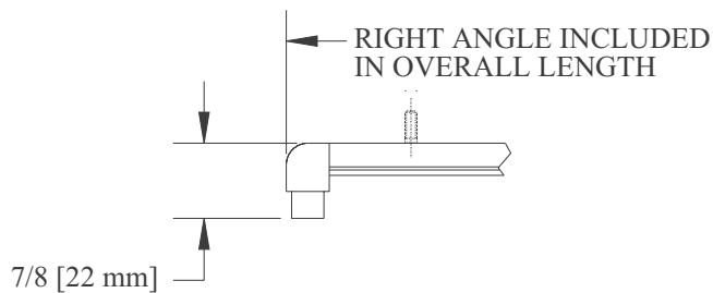
OPTIONAL RIGHT ANGLE CABLE EXIT
