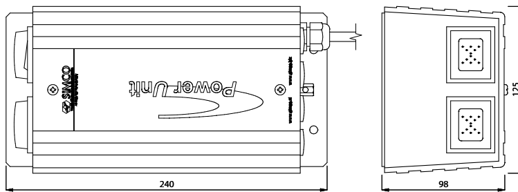
Technical drawing A Unit
